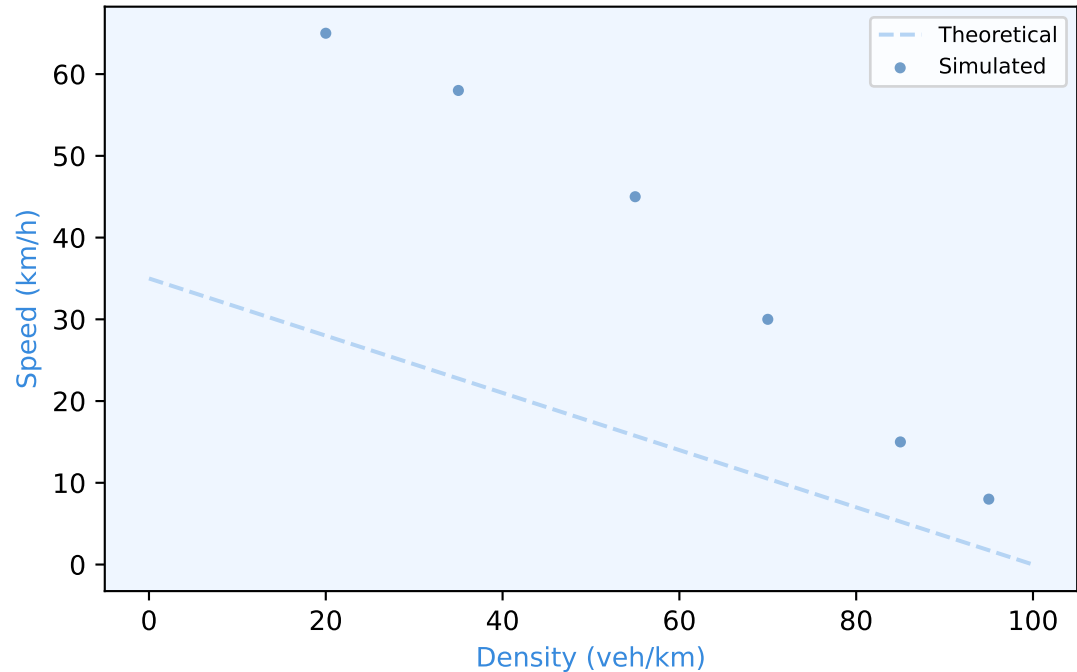
Speed vs Density
